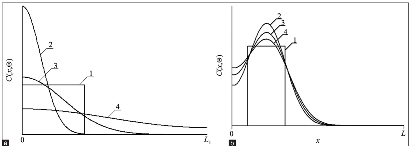
Figure 4: (a) Distributions of concentration of infused dopant in depth of heterostructure from Figure 1 for different values of annealing time (curves 2–4) and idealized step-wise approximation (curve 1). Increasing of number of curve corresponds to increasing of annealing time, (b) Distributions of the concentration of implanted dopant in depth of heterostructure from Figure 1 for different values of annealing time (curves 2–4) and idealized step-wise approximation (curve 1). Increasing of number of curve corresponds to increasing of annealing time
