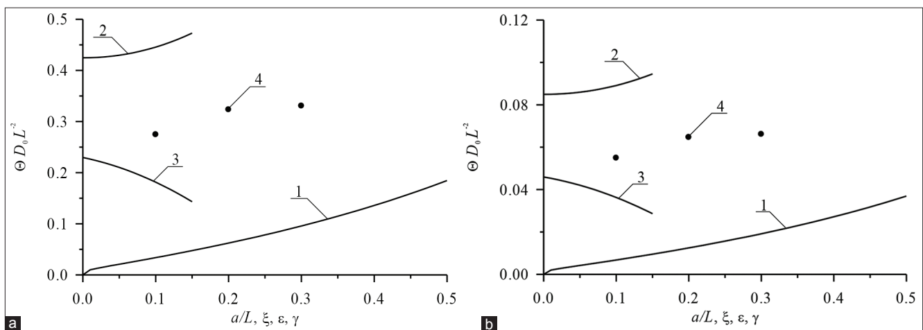
Figure 5: (a) Dimensionless optimal annealing time of infused dopant as a function of several parameters. Curve 1 describes the dependence of the annealing time on the relation a/L and \xi=\gamma=0 for equal to each other values of dopant diffusion coefficient in all parts of heterostructure. Curve 2 describes the dependence of the annealing time on value of parameter \varepsilon for a/L=1/2 and \xi=\gamma=0 . Curve 3 describes the dependence of the annealing time on value of parameter \xi for a/L=1/2 and \varepsilon=\gamma=0 . Curve 4 describes the dependence of the annealing time on value of parameter \gamma for a/L=1/2 and \varepsilon=\xi=0 , (b) Dimensionless optimal annealing time of implanted dopant as a function of several parameters. Curve 1 describes the dependence of the annealing time on the relation a/L and \xi=\gamma=0 for equal to each other values of dopant diffusion coefficient in all parts of heterostructure. Curve 2 describes the dependence of the annealing time on value of parameter \varepsilon for a/L=1/2 and \xi=\gamma=0 . Curve 3 describes the dependence of the annealing time on value of parameter \xi for a/L=1/2 and \varepsilon=\gamma=0 . Curve 4 describes the dependence of the annealing time on value of parameter \gamma for a/L=1/2 and \varepsilon=\xi=0
