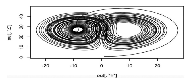
Figure 1: Lorenz attractor that appears in form of chaos about the world climate – plotted from R-studio software
