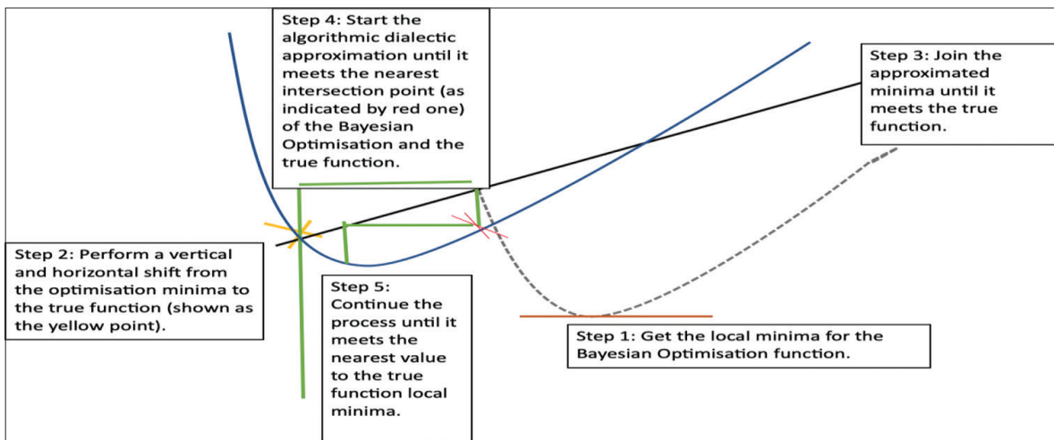
Figure 3: Steps in finding the true local minima and the intersection (optimal) point (of the HKLam theory and Lorenz system) between the Bayesian optimization function and the model of the true function. In fact, the present method (modified from fixed-point algorithm [28] ) convergent rate is clearly much faster than the point-wise gradient descent algorithm
