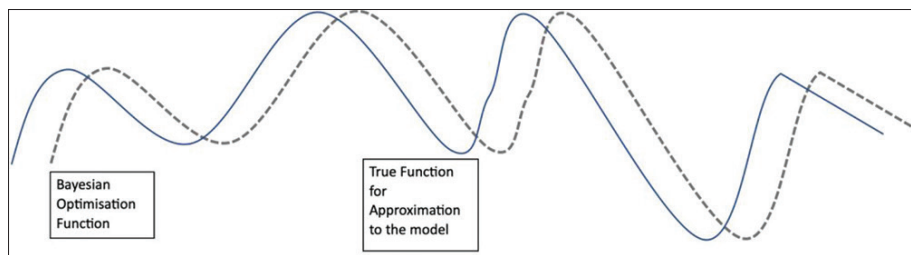
Figure 2: Using the Bayesian optimization function to approximate the model of the true function [24]
