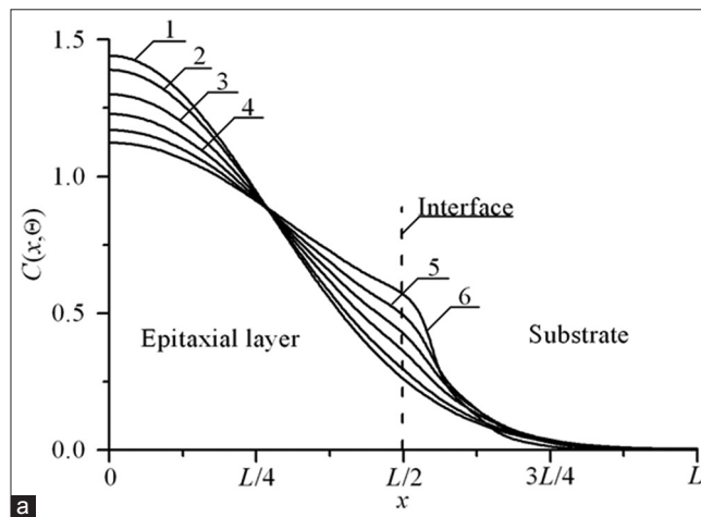
Figure 2: (a) Dependences of concentration of dopant, infused in heterostructure from Figure 1, on coordinate in direction, which is perpendicular to interface between epitaxial layer substrate. Difference between values of dopant diffusion coefficient in layers of heterostructure increases with increasing of number of curves. Value of dopant diffusion coefficient in the epitaxial layer is larger, than value of dopant diffusion coefficient in the substrate
