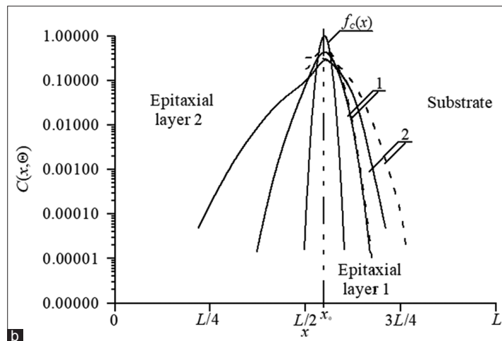
Figure 3: (b) Calculated distributions of implanted dopant in epitaxial layers of heterostructure. Solid lines are spatial distributions of implanted dopant in system of two epitaxial layers. Dashed lines are spatial distributions of implanted dopant in one epitaxial layer. Annealing time increases with increasing of number of curves
