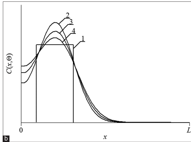
Figure 4: (b) Distributions of concentration of implanted dopant in depth of heterostructure from Figure 1 for different values of annealing time (curves 2-4) and idealized step-wise approximation (curve 1). Increasing of number of curve corresponds to increasing of annealing time
