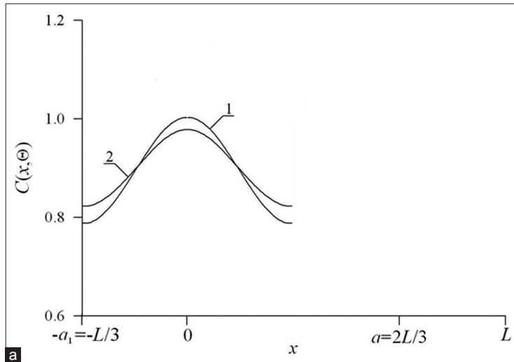
Figure 3: (a) Distributions of concentration of dopant, infused in average section of epitaxial layer of heterostructure from Figure 1 in direction parallel to interface between epitaxial layer and substrate of heterostructure. Difference between values of dopant diffusion coefficients increases with increasing of number of curves. Value of dopant diffusion coefficient in this section is smaller, than value of dopant diffusion coefficient in nearest sections
