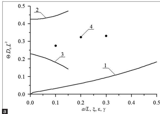
Figure 5: (a) Dimensionless optimal annealing time of infused dopant as a function of several parameters. Curve 1 describes the dependence of the annealing time on the relation a/L and \zeta = \gamma = 0 for equal to each other values of dopant diffusion coefficient in all parts of heterostructure. Curve 2 describes the dependence of the annealing time on value of parameter \epsilon for a/L=1/2 and \zeta = \gamma = 0 . Curve 3 describes the dependence of the annealing time on value of parameter \zeta for a/L=1/2 and \epsilon = \gamma = 0 . Curve 4 describes the dependence of the annealing time on value of parameter \gamma for a/L=1/2 and \epsilon = \zeta = 0
