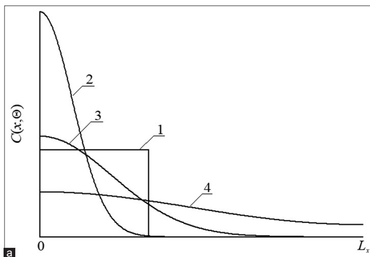
Figure 4: (a) Distributions of concentration of infused dopant in depth of heterostructure from Figure 1 for different values of annealing time (curves 2-4) and idealized step-wise approximation (curve 1). Increasing of number of curve corresponds to increasing of annealing time
