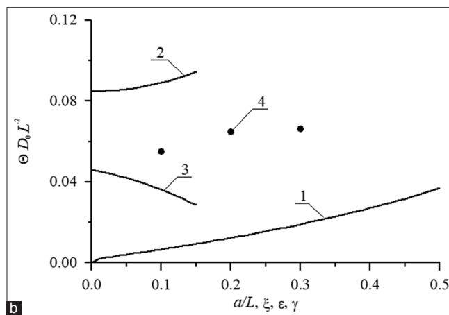
Figure 5: (b) Dimensionless optimal annealing time of implanted dopant as a function of several parameters. Curve 1 describes the dependence of the annealing time on the relation a/L and \zeta = \gamma = 0 for equal to each other values of dopant diffusion coefficient in all parts of heterostructure. Curve 2 describes the dependence of the annealing time on value of parameter \epsilon for a/L=1/2 and \zeta = \gamma = 0 . Curve 3 describes the dependence of the annealing time on value of parameter \zeta for a/L=1/2 and \epsilon = \gamma = 0 . Curve 4 describes the dependence of the annealing time on value of parameter \gamma for a/L=1/2 and \epsilon = \zeta = 0
