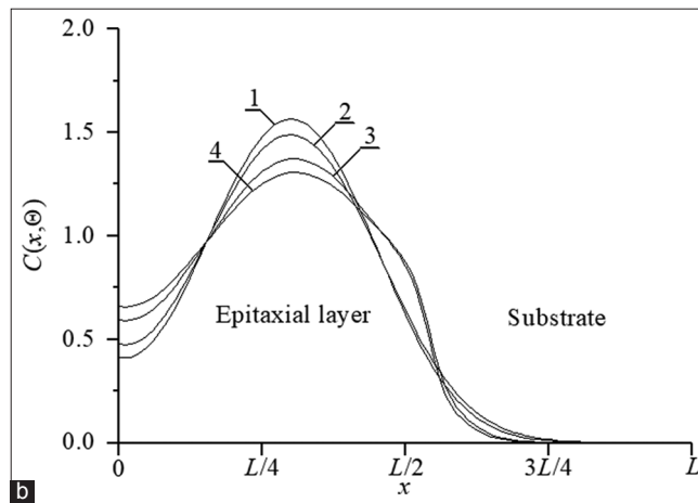
Figure 2: (b) Dependences of concentration of dopant, implanted in heterostructure from Figure 1, on coordinate in direction, which is perpendicular to interface between epitaxial layer substrate. Difference between values of dopant diffusion coefficient in layers of heterostructure increases with increasing of number of curves. Value of dopant diffusion coefficient in the epitaxial layer is larger, than value of dopant diffusion coefficient in the substrate. Curve 1 corresponds to homogenous sample and annealing time \Theta = 0.0048 (L_x^2 + L_y^2 + L_z^2)/D_0 . Curve 2 corresponds to homogenous sample and annealing time \Theta = 0.0057 (L_x^2 + L_y^2 + L_z^2)/D_0 . Curves 3 and 4 correspond to heterostructure from Figure 1; annealing times \Theta = 0.0048 (L_x^2 + L_y^2 + L_z^2)/D_0 and \Theta = 0.0057 (L_x^2 + L_y^2 + L_z^2)/D_0 , respectively
